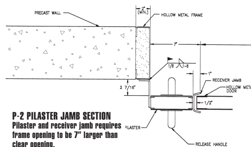
DETAIL C - PILASTER P2
