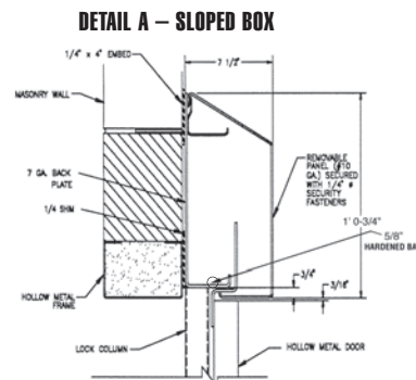
COVER BOX SECTION 7-1/2" deep x 1' - 0-3/4" tall cover box field welded 1" on 8" top and bottom.
