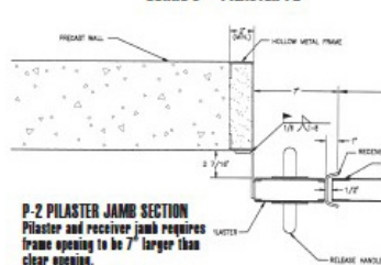
DETAIL C - PILASTER P2
