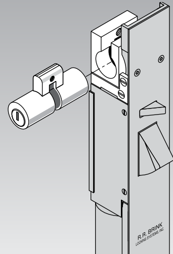
Europrofile key cylinder option – EURO
