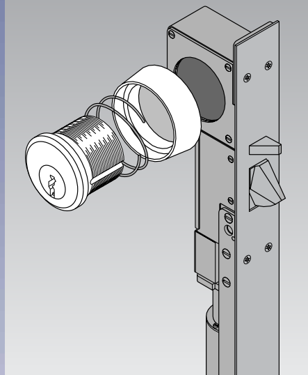
Europrofile key cylinder option – EURO
