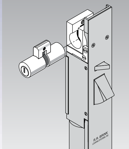
Europrofile key cylinder option – EURO
